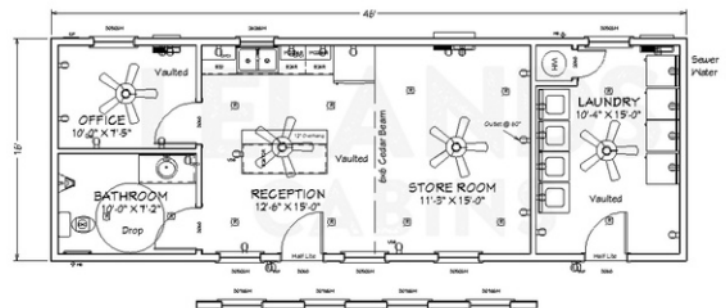
OFFICE & LAUNDRY 16X46 / 736 SQ FT
